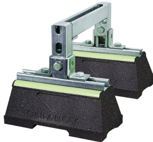
Raised Bridge Medium Support with 2 CBN Bases & 1-5/8" (41mm) Pre-Galv or Hot Dip Galv. Steel Channel
