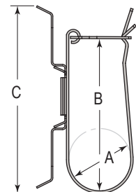
CBMTRH Series Cush-A-Block Mini with Raised TRH Hanger Clamp for Cable Runs or Insulated Pipe & Tubing
