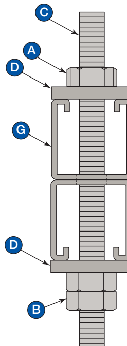
Double Section Perforated Channel
