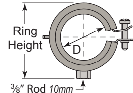
CBMPH Series Cush-A-Block Mini with Raised SPH Cush-A-Ring Clamp for Copper or Steel Tube or Pipe
